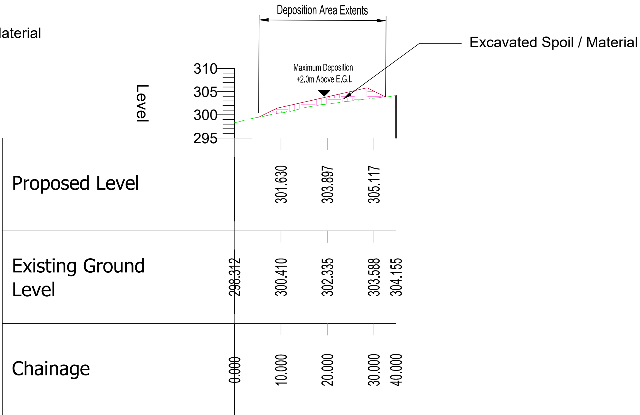
SPOIL DEPOSITION AREA -02_ALIGNMENT-B - LONGSECTION SCALE: H 1:1000,V 1:1000. DATUM: 270.000
