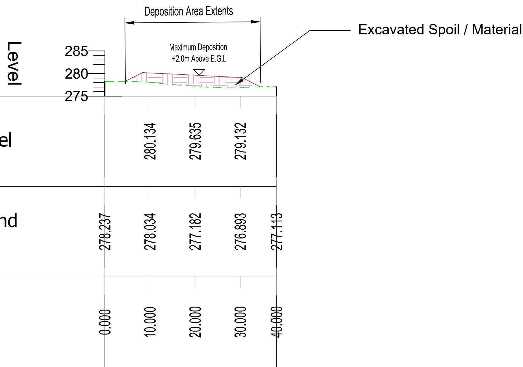
SPOIL DEPOSITION AREA -01_ALIGNMENT-B - LONGSECTION SCALE: H 1:500,V 1:500. DATUM: 270.000
