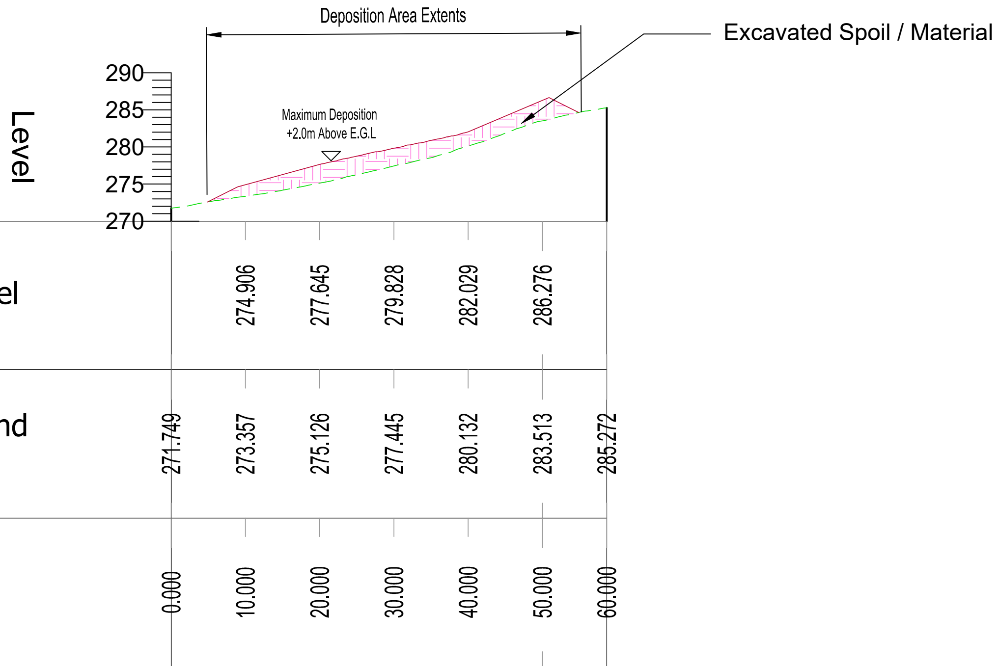
SPOIL DEPOSITION AREA -01_ALIGNMENT-A - LONGSECTION SCALE: H 1:500,V 1:500. DATUM: 270.000
