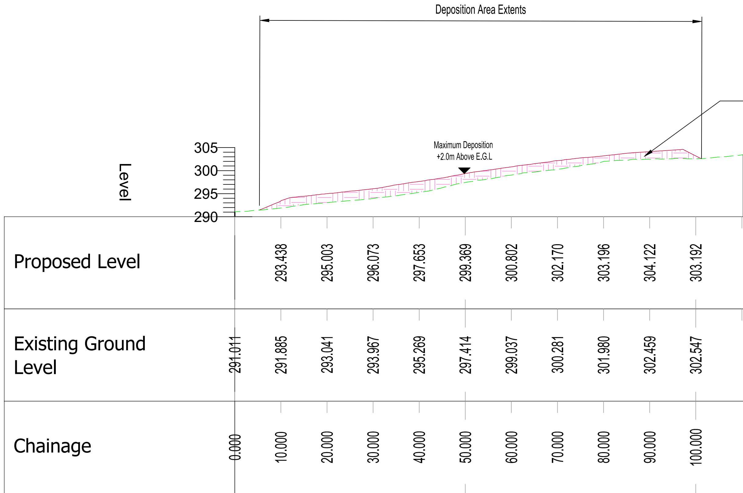
SPOIL DEPOSITION AREA -02_ALIGNMENT-A - LONGSECTION SCALE: H 1:500,V 1:500. DATUM: 270.000
