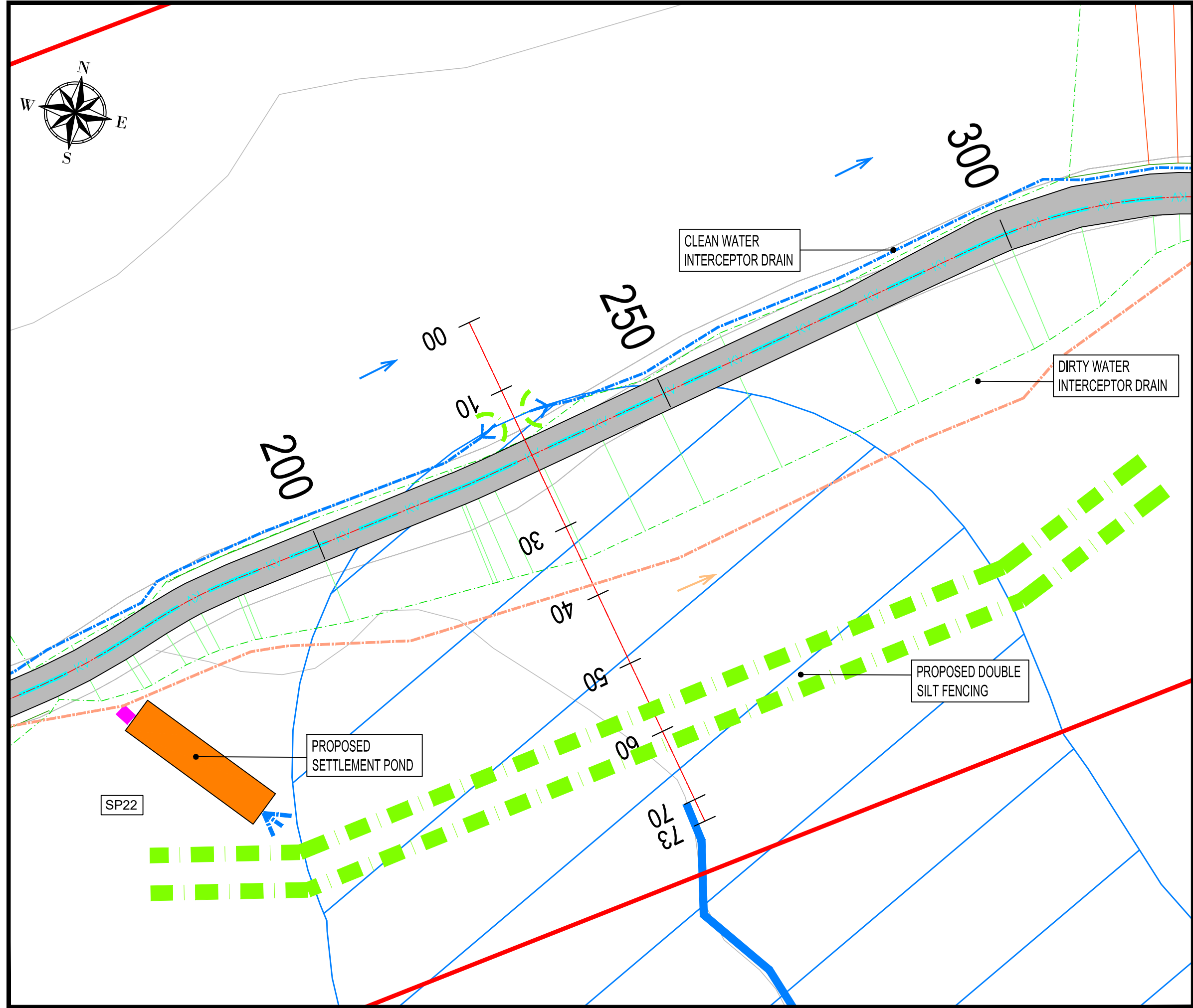
Site Layout Plan Scale 1:500(A1)
